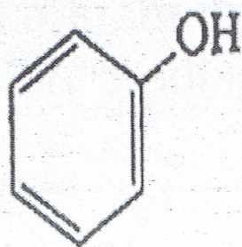
Phenol
