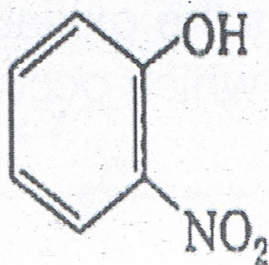
2-Nitrophenol
