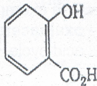
Salicylic acid
